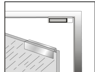
Demonstration of UL Bracket Installation
